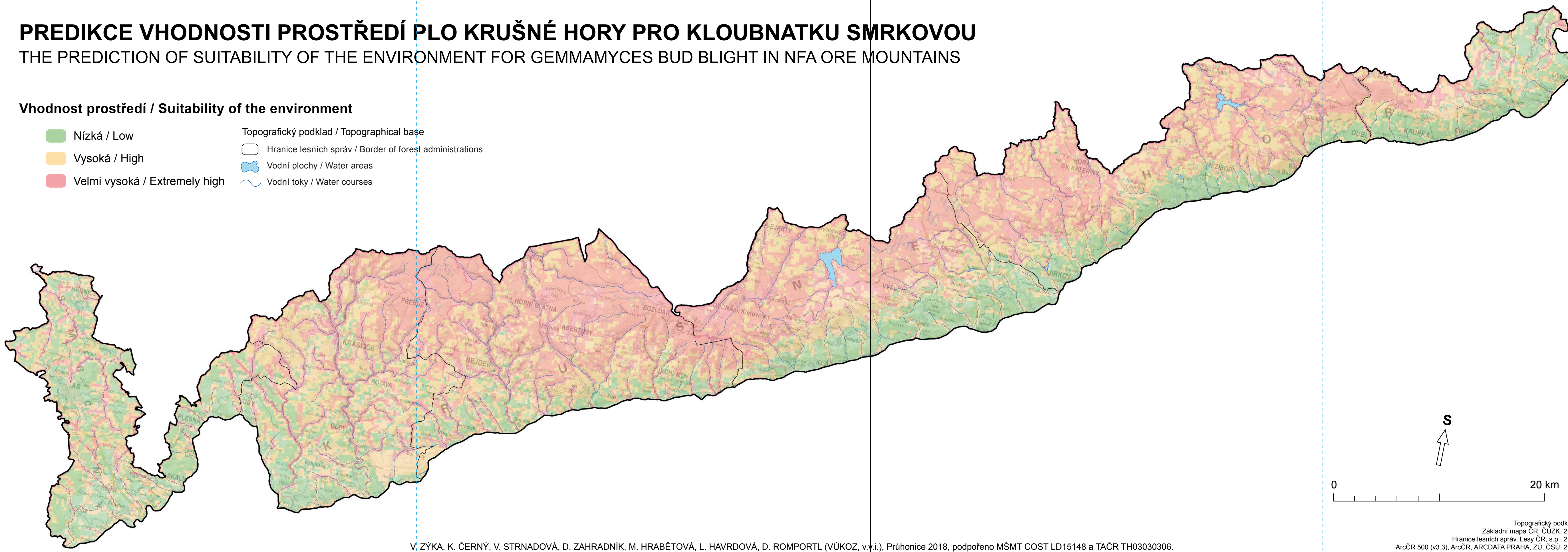
Obr. 20: Vhodnost prostředí pro kloubnatku smrkovou v PLO Krušné hory Fig. 20: A suitability of the environment for Gemmamyces bud blight in the NFA Ore Mountains
